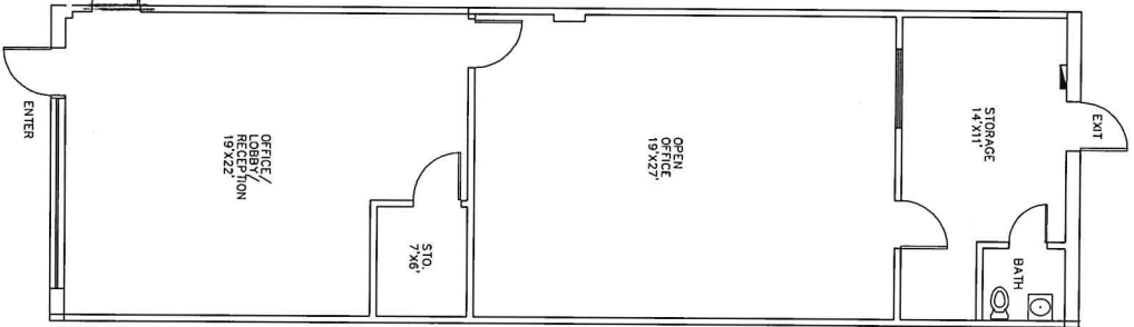
2529 BERNADETTE FLOOR PLAN SCALE: 1/4"=1'-0"
